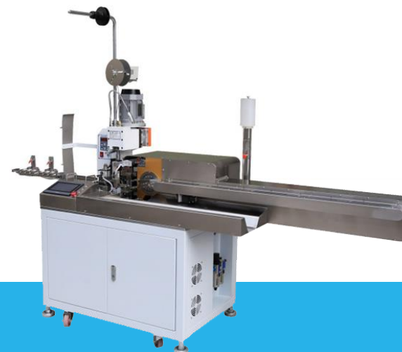
全自动裁线、剥线、捻线沾锡压接一体机 Automatic all-in-one machine for cutting, stripping, tinning, crimping
